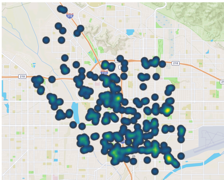
Figure 12: Example of plotting an enhancement-based dataset (TVOCs) as a heatmap. In this type of map, the density of individual enhancement events are shown, where the brighter colors indicate a higher density of detected enhancements. In this example, data collected over a 3 month period in San Bernardino, CA are shown. Map data © Mapbox , © OpenStreetMap .
